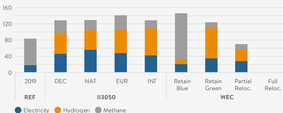
Figure 30. Total demand of the four energy-intensive industries sectors in 2040 (TWh)
