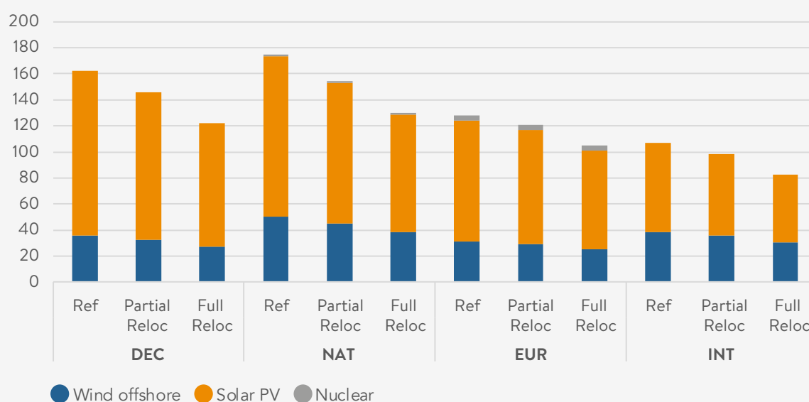
Figure 34. Impact on electricity supply capacities (GW)
