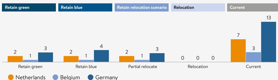
Figure 26. Total CO 2 -emissions for refining per country for the different scenarios (Mt)
