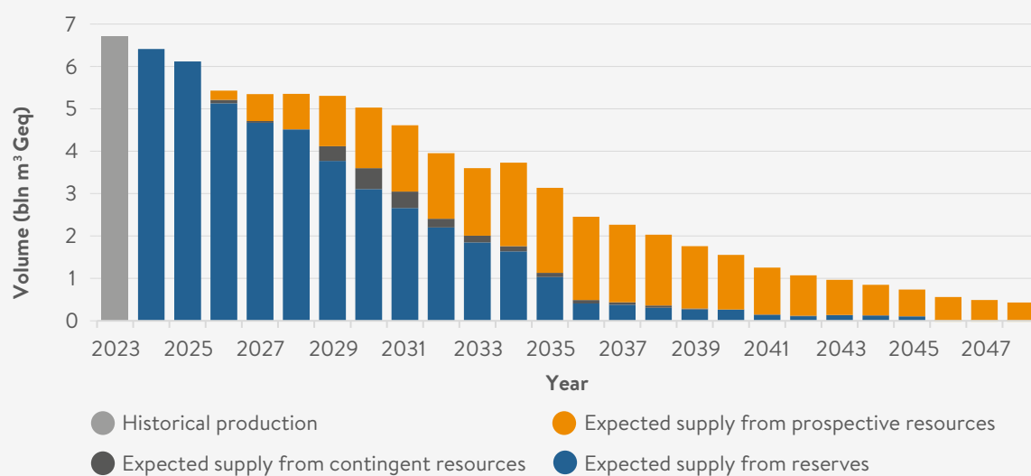
Figure 35. Expected gas production from small fields at the Dutch part of the North Sea
