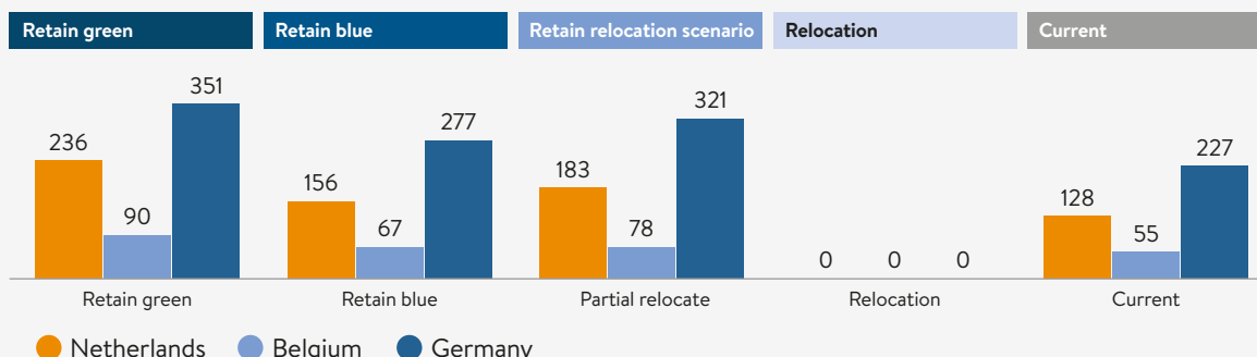
Figure 25. Total energy consumption for refining per country for different scenarios (in PJ)
